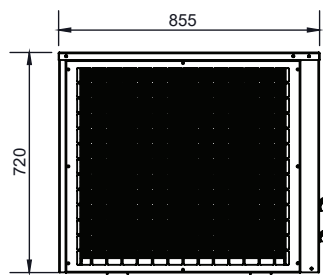
Outdoor Unit - ODU
